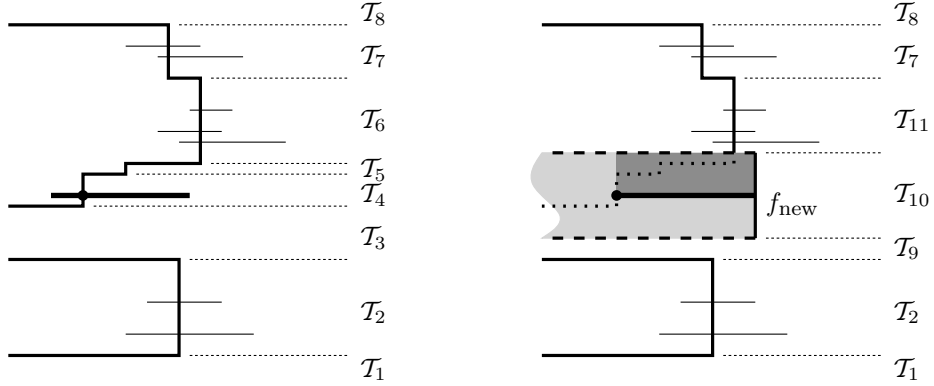
Fig. 20. When the fat horizontal segment s from H_{\text{int}} is chosen, the frontier becomes the right envelope of f_{\text{new}} and the old frontier. The new label is dark grey. The grey range (light and dark) is the one with which queries in the priority search trees are done.
