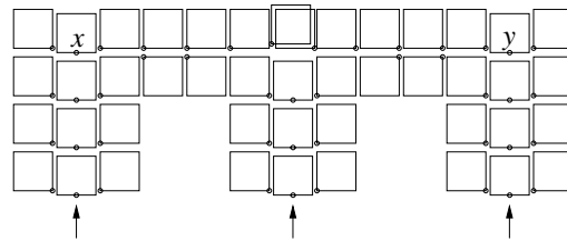
Fig. 15. Clause with pressure from three variables.
