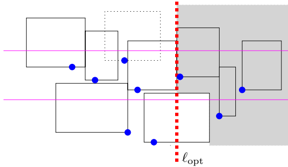
Fig. 22. An optimal solution for the same points as in the figure above.
