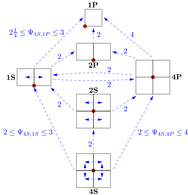
Fig. 11. Ratios between some label placement models. From top to bottom: the one-position, two-position, top-slider (left), four-position (right), two- and four-slider model
