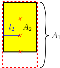
Fig. 7. If M_1 can be slid into M_2 then the leftmost M_2 -label l_2 cannot intersect more than two M_2 -labels.
