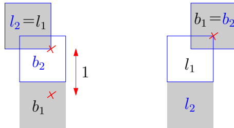
Fig. 6. If M_1 can be flipped into M_2 then the leftmost M_2 -label l_2 (solid edges) cannot intersect more than one M_2 -label b_2 . (The corresponding non-intersecting M_1 -labels are shaded.)
