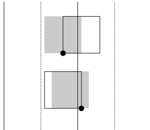
Fig. 9. After removing M_1 -labels intersecting the odd lines (dashed), the remaining M_1 -labels (shaded) are corner slid to intersect an even line (solid). This results in a valid M_2 -labeling.
