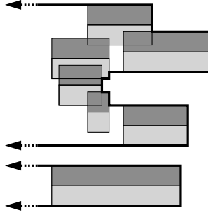
Fig. 18. Frontier of the placed labels (dark grey) and their lowered copies (light grey).
