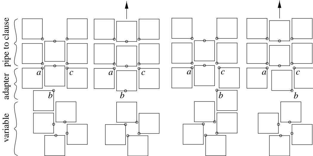
Fig. 16. Adapters for unnegated literals exert pressure when a variable is set to false .
