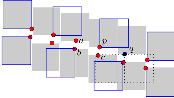
Fig. 8. If M_1 can be slid into M_2 then the M_1 - M_2 -ratio approaches 2. Here we chose M_1 to be the two-slider model (shaded labels) and M_2 to be the four-position model (solid edges).
