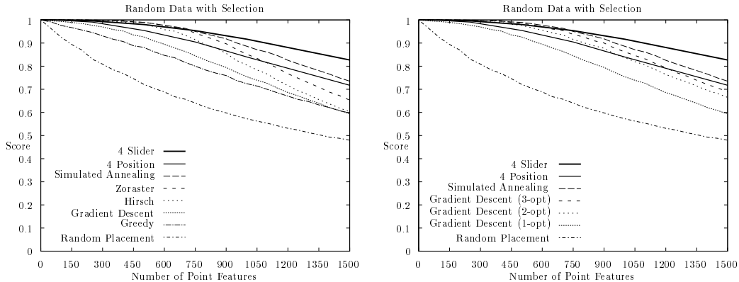
Fig. 27. Comparison of the four-position and four-slider algorithm to other labeling algorithms.
