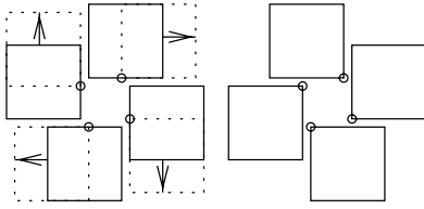
Fig. 12. Label placements encoding true and false .
