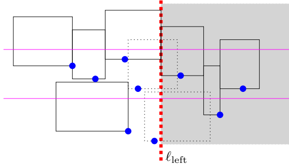
Fig. 21. Leftmost label placement for a subset of k = 4 labels and t = 2 lines.
