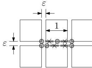
Fig. 5. 3/2 is a lower bound on the ratio between the two- or four-slider and any fixed-position model
