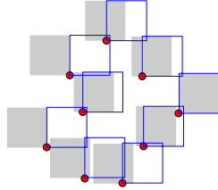
Fig. 10. Sliding top-slider labels (shaded) to the right into one-position labels (solid edges) can create 9-cycles in the resulting conflict graph of one-position labels.
