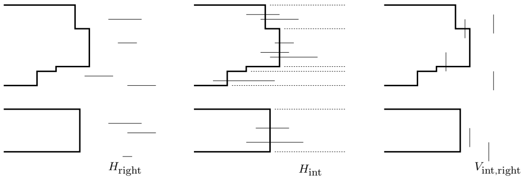
Fig. 19. The sets H_{\text{right}} , H_{\text{int}} , and V_{\text{int, right}} . The dashed lines in the middle picture separate the segments of H_{\text{int}} that are in different red-black trees \mathcal{T}_i .
