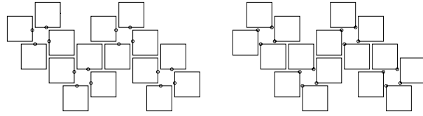
Fig. 13. Zig-zagging cluster patterns model a variable; the labels its Boolean value.
