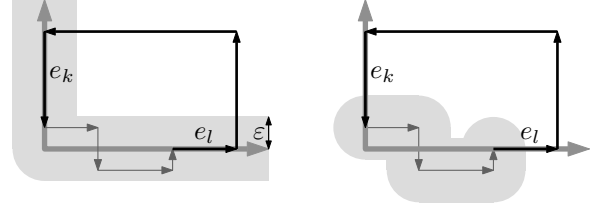
Figure 5: Feasibility of shortcut (e_k, e_l) . \varepsilon -Buffers are shaded. The bold gray arrows indicate the L-shape defined by (e_k, e_l) .
