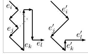
Figure 3: Applying shortcuts (e_i, e_j) and (e_k, e_l) results in a simple polygon, though (e_i, e_j) is not feasible alone.
