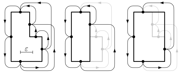
Figure 13: A building with two feasible simplifications.
