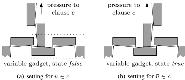
Figure 11: A connector that is attached to variable u . The region in the dotted rectangle is shown in Fig. 9 in detail.
