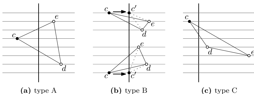
Fig. 4: The three types of faces.
