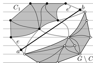
Fig. 3: Split along ab .
