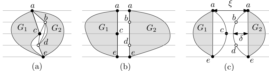
Fig. 8: (a) Shortcuts in the separating path—the left path is ace , the right path abde , (b) recursive drawing of G_1 and G_2 , (c) the two parameters \xi and \delta .
