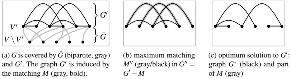
Fig. 2: Partitioning the input graph and the optimum solution in the proof of Theorem 9
